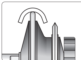
The Profiled Leather Honing wheel LA-120 copes with all size of gouges. The generous space between the discs allows honing even of large roughing gouges, here size 32 mm ( 1\frac{1}{4} " ).
