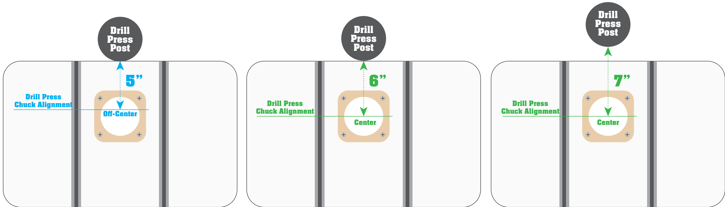
10" Drill Press
